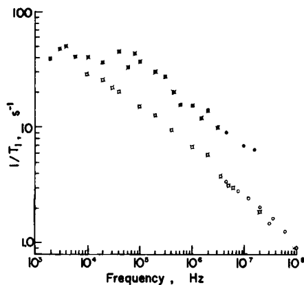
FIGURE 1 Proton (○) and deuteron (●) relaxation rates of muscle water at 25°C as functions of Larmor frequency. The data marked with crosses were taken at the IBM Watson Research Center (see acknowledgment). The deuteron data at 4.5, 9.2, and 15.4 MHz were obtained by using the leg muscle from partially deuterated mice (ca. 30%, ref. 5). Because of intensity problems below 4 MHz, the partially deuterated muscle samples were further soaked in a modified Krebs solution with D 2 O as solvent for 1 hr to increase the deuterium content of muscle water. Bathing the muscle in normal Krebs solution increased the total water content slightly; therefore the modified Krebs solution contained 25 g/liter glucose so that the total water content was kept the same as in fresh muscle. Muscle samples treated this way had the same T_1 values as fresh muscle samples.
