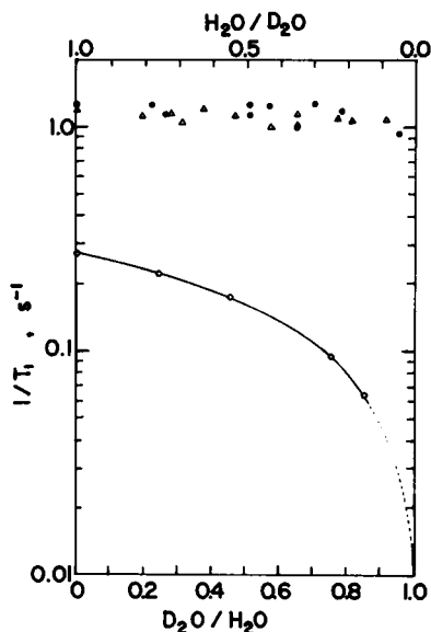
FIGURE 3 Proton relaxation rates of bulk water (○), water in mouse muscle (Δ), and brain (●) at 25°C and 35 MHz as functions of isotope substitution. The samples were bathed in Krebs solution with different D 2 O contents for 1 h. For samples containing more than 70% D 2 O, the proton magnetization decay was slightly nonexponential because of the contribution of organic protons (B. M. Fung, to be published); T_1 was taken from the slowly decaying part of the plot. T_1 data for bulk H 2 O were obtained from ref. 10.
